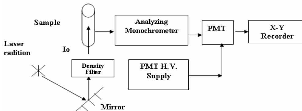
Fig. (1): Schematic diagram of fluorescence spectra system.
